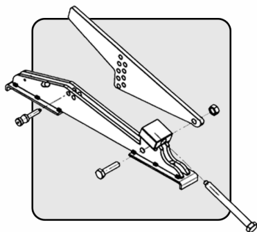
010059 - Clamping system
